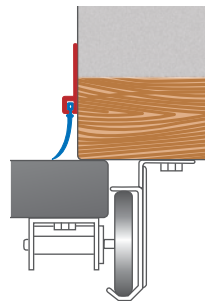
A0282-MI-W/B0772-00-W (3" STANDARD BRUSH SEAL, PG.5)
