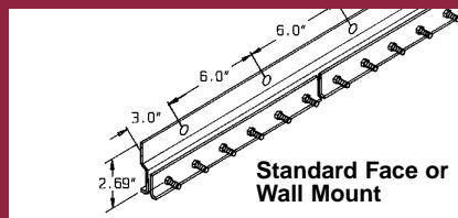
Standard Jamb Header Mount
